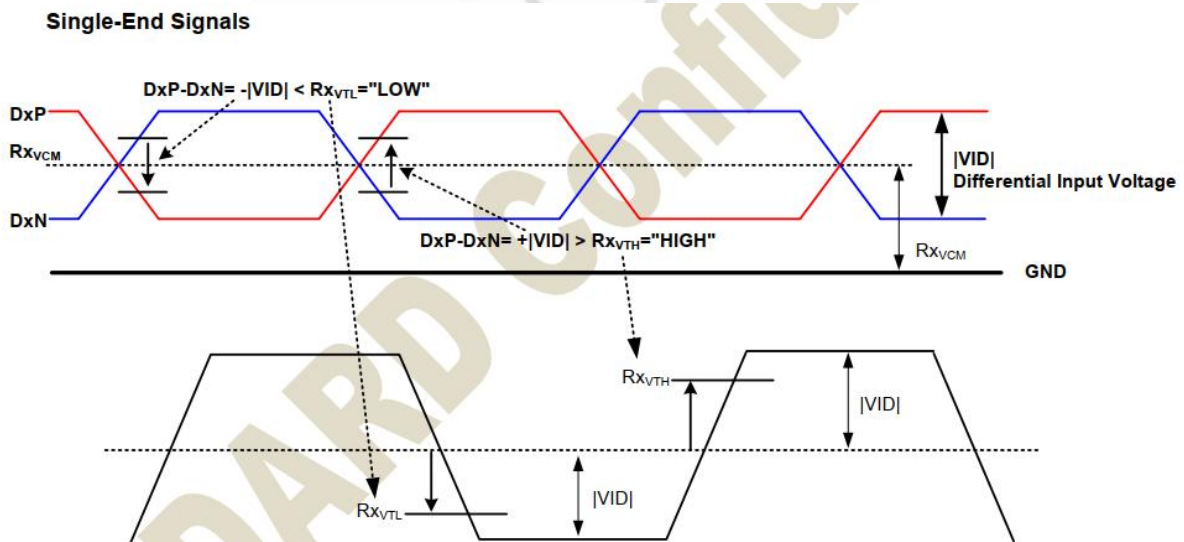
Figure 11.1: LVDS input timings
